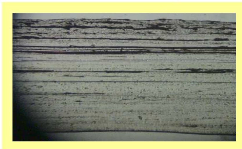
Section of a HDPE container wall with Quoral barrier layer
